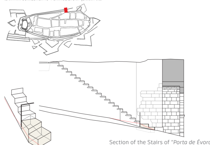
Section of the Stairs of "Porta de Évora"
