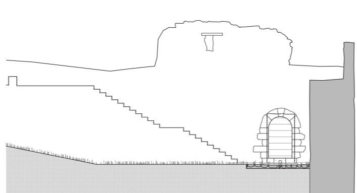
Frontal Elevation of "Casa do Inquisidor-Mor"
