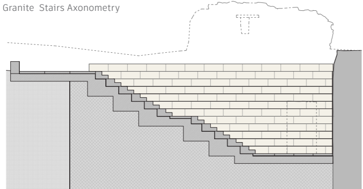
Section of the Stairs of "Casa do Inquisidor-Mor"
